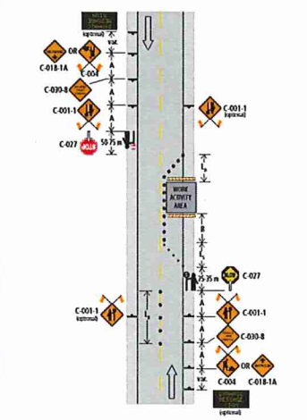
Figure 7.A: Lane Closure with TCPs – Single Lane Alternating – Short and Long Duration
