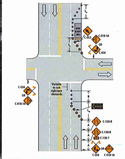
Figure 11.B: Right Lane Closure (Far Side) – Multilane Intersection – Short and Long Duration
